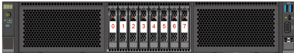
Figure 5-29 Drive numbers
