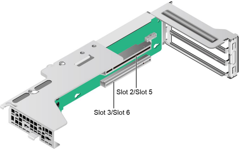
Figure 5-57 PCIe riser card 1 (BC16M03PRUL-supporting the full-length and dual-width GPU)
