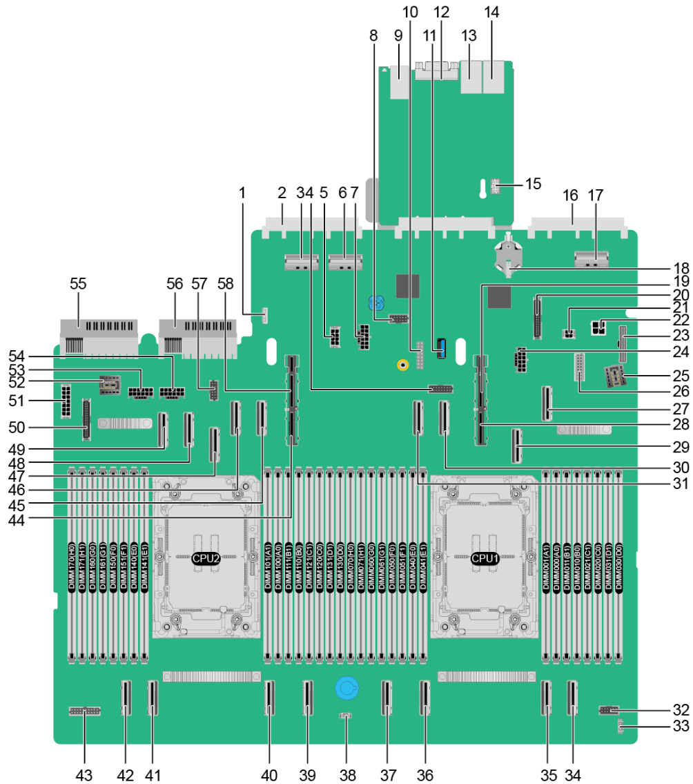
Figure 5-61 Mainboard
