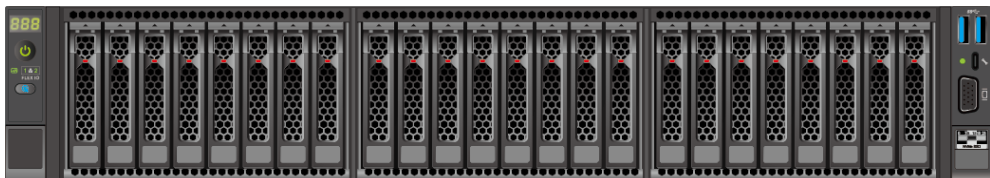
Figure 5-18 24 x 2.5" drive configuration
