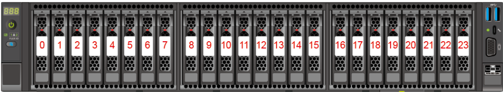
Figure 5-45 Drive numbers
