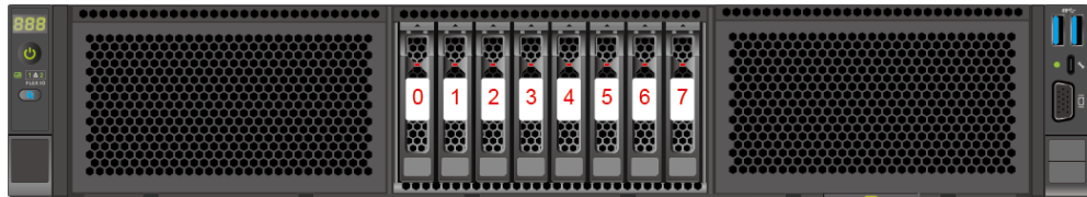
Figure 5-30 Drive number 1
