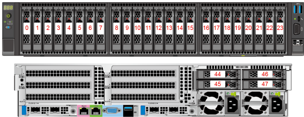
Figure 5-41 Drive number
