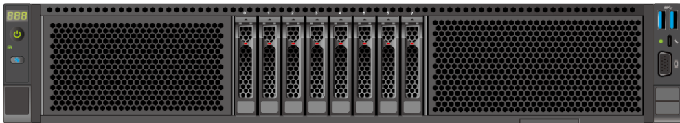
Figure 5-2 8 x 2.5" drive configuration 2
