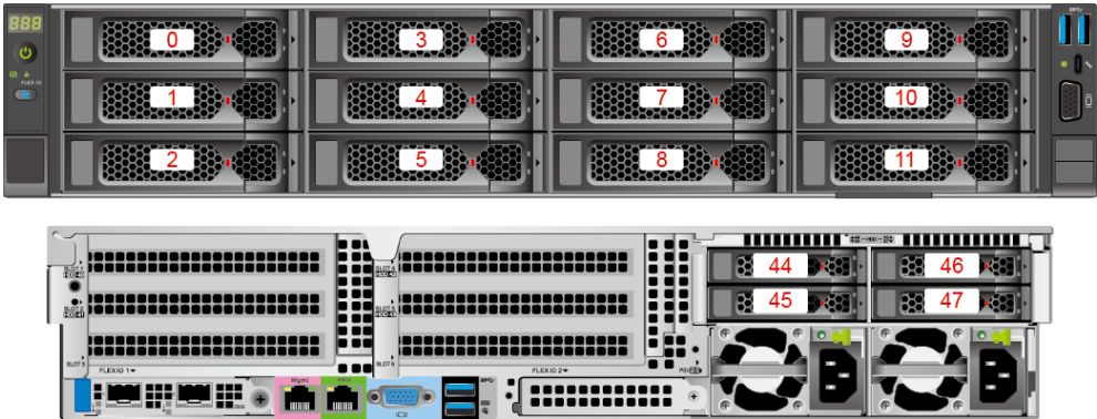
Figure 5-31 Drive numbers 1
