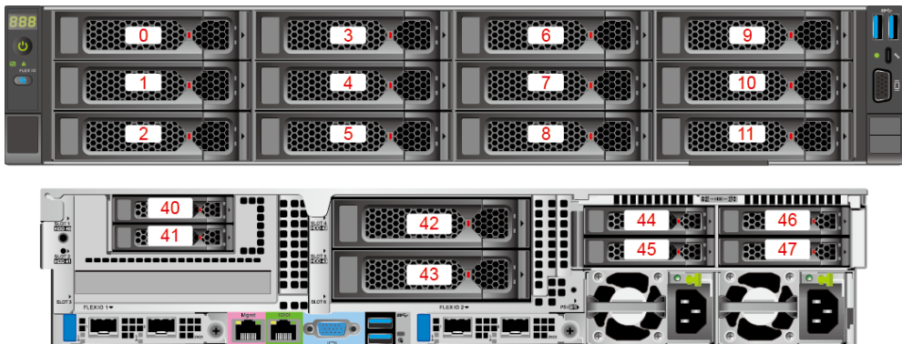
Figure 5-26 Drive number 2
