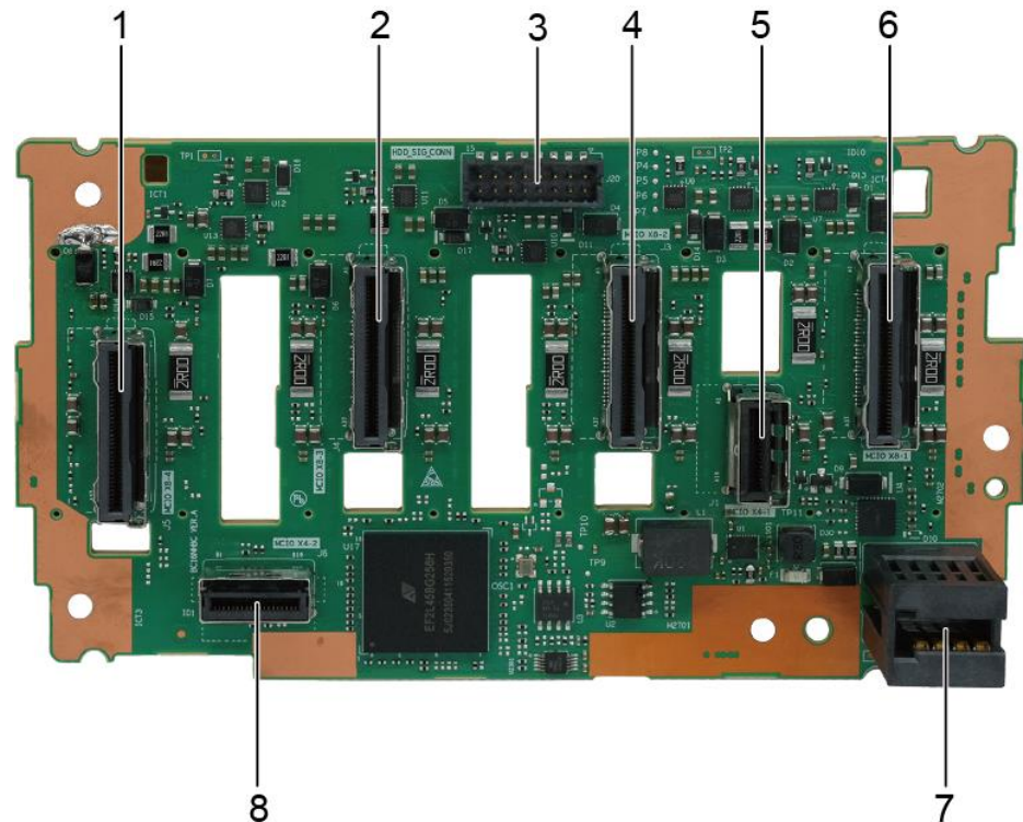
Figure 5-62 8 x 2.5" SAS/SATA/NVMe 3cage drive backplane
