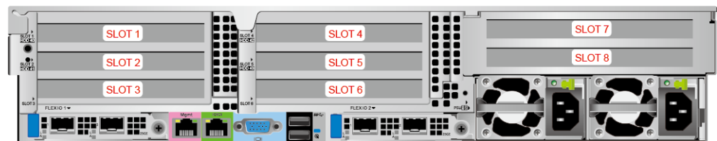
Figure 5-48 PCIe slots
