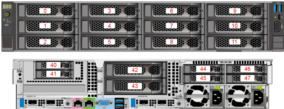
Figure 5-33 Drive numbers 2
