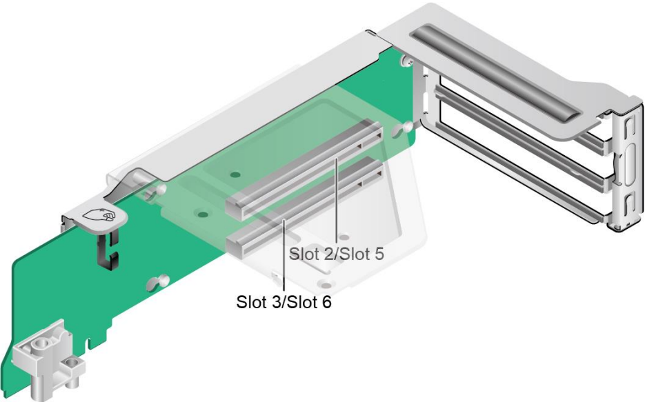
Figure 5-58 PCIe riser card 41 (BC16M02PRUKA-supporting the cable card)
