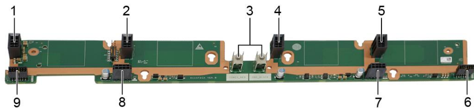
Figure 5-71 Fan board
