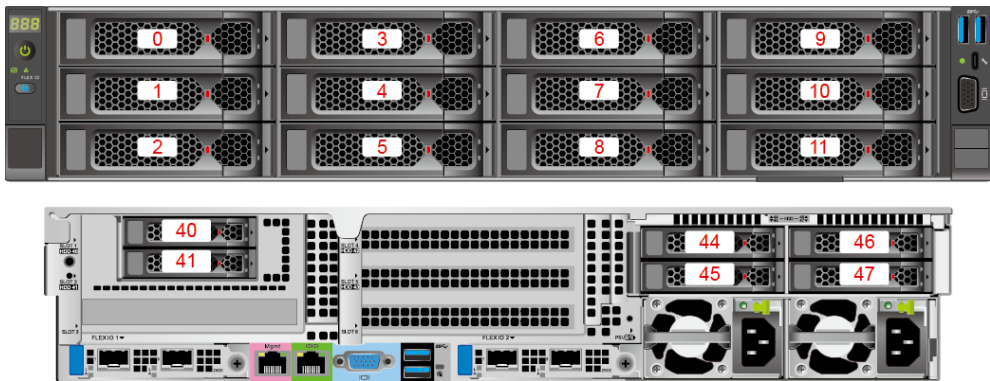
Figure 5-35 Drive numbers
