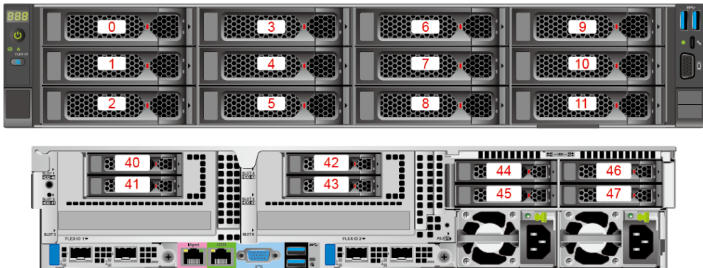
Figure 5-25 Drive number 1
