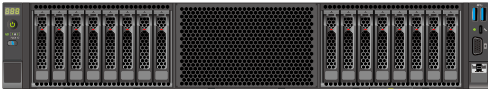
Figure 5-11 16 x 2.5" drive configuration 2
