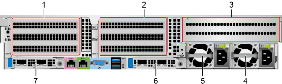
Figure 5-19 Rear panel
