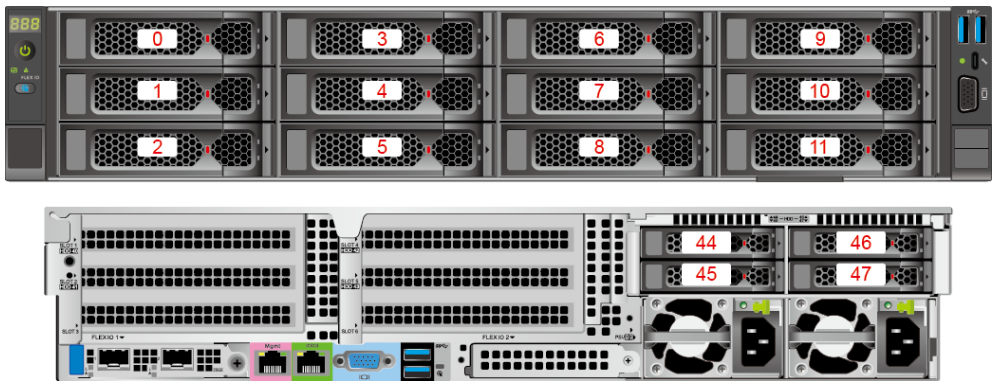
Figure 5-34 Drive numbers 3
