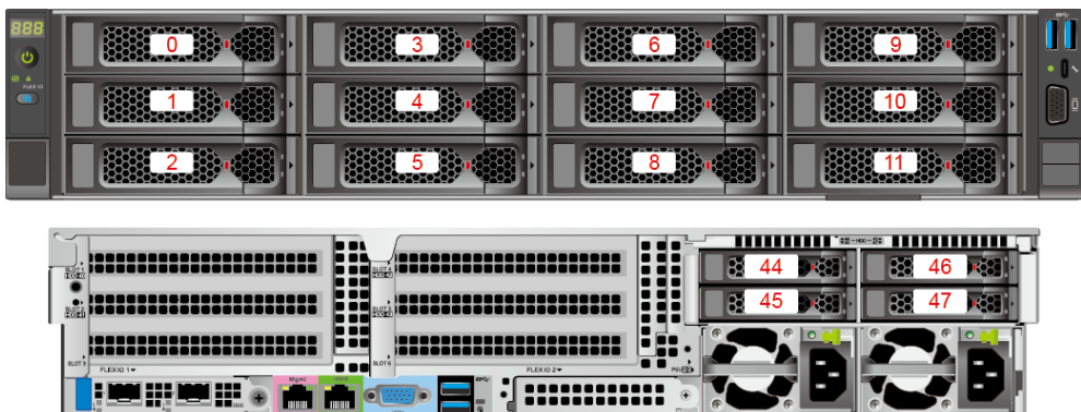
Figure 5-27 Drive number 3
