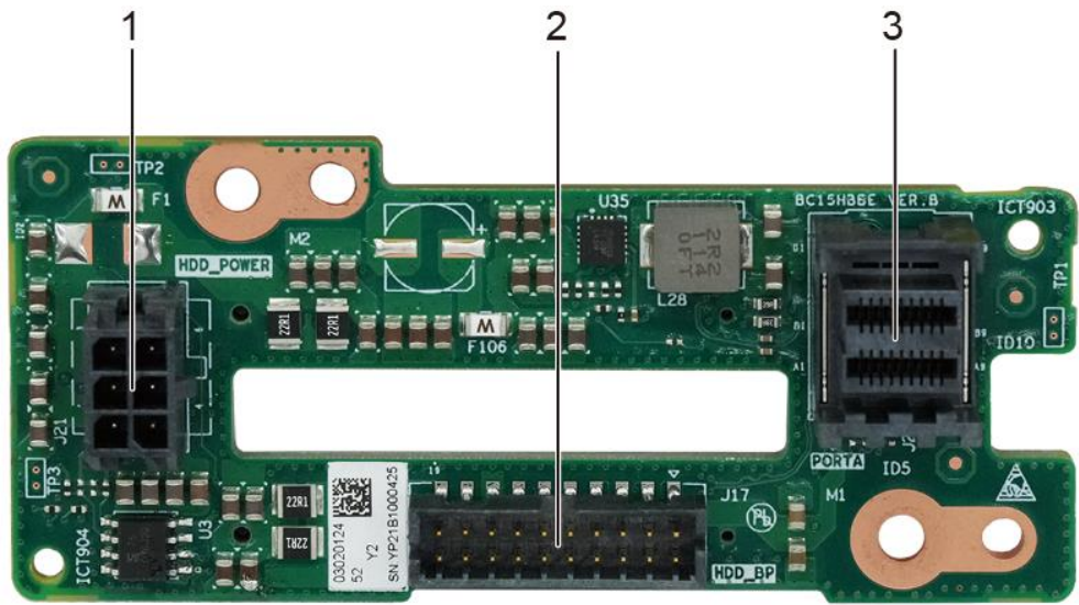
Figure 5-67 2 x 2.5" drive backplane
